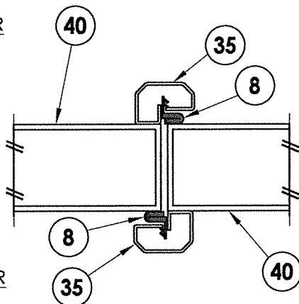
3 HORIZONTAL CROSS SECTION 4 Outswing Shown (Inswing Similar)
