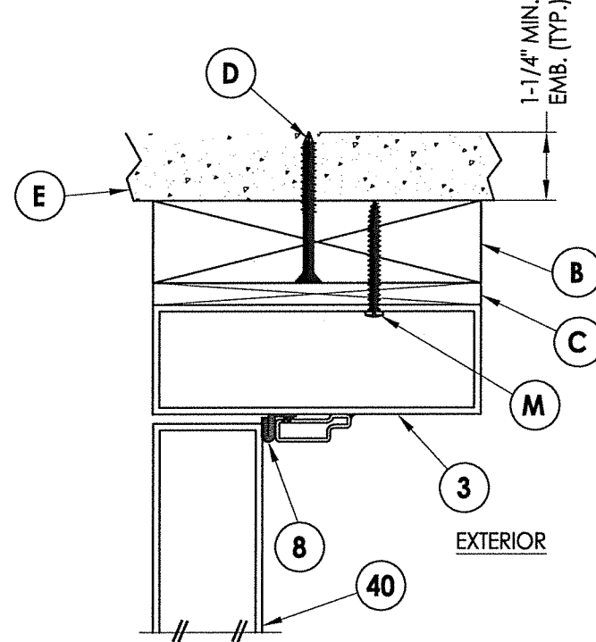
7 HORIZONTAL CROSS SECTION 4 Inswing Shown (Inswing Similar) 2X Buck Masonry Anchoring
