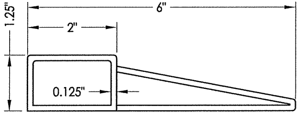
36 THRESHOLD Inswing
