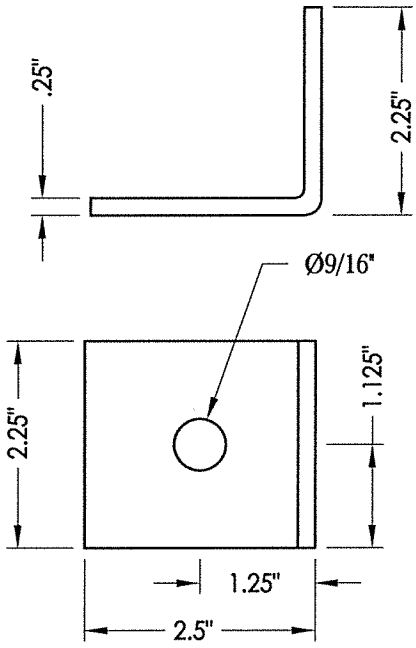
15 ANCHORING BRACKET
