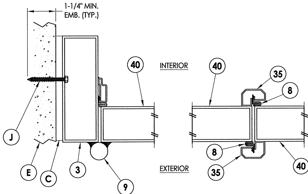
2 HORIZONTAL CROSS SECTION 4 Outswing Shown (Inswing Similar) Direct to Masonry Anchoring
