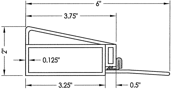
39 THRESHOLD Outswing
